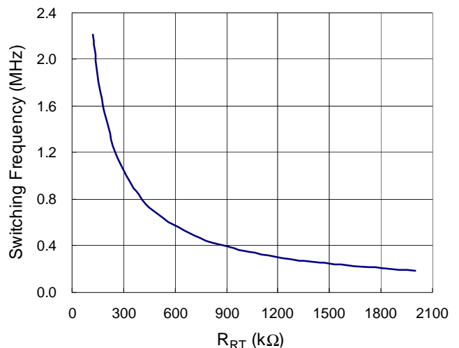
Figure 2. Switching Frequency vs. RT Resistor
