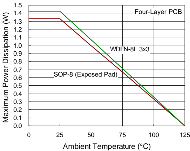
Figure 3. Derating Curve for the RT8065 Package
